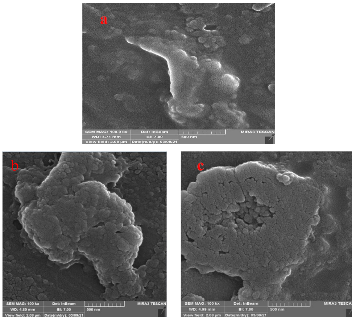
Figure 6: FE-SEM micrographs of TiO 2 NPs synthesised with laser energy of (a) 80 mJ, (b) 120mJ, and (c) 160mJ at 100 pulses.
