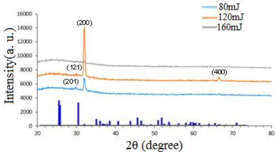
Figure 5: XRD spectra of the \text{TiO}_2 NPs prepared at different laser energy standard XRD peaks positions pattern of Brookite \text{TiO}_2 placed on x-axis
