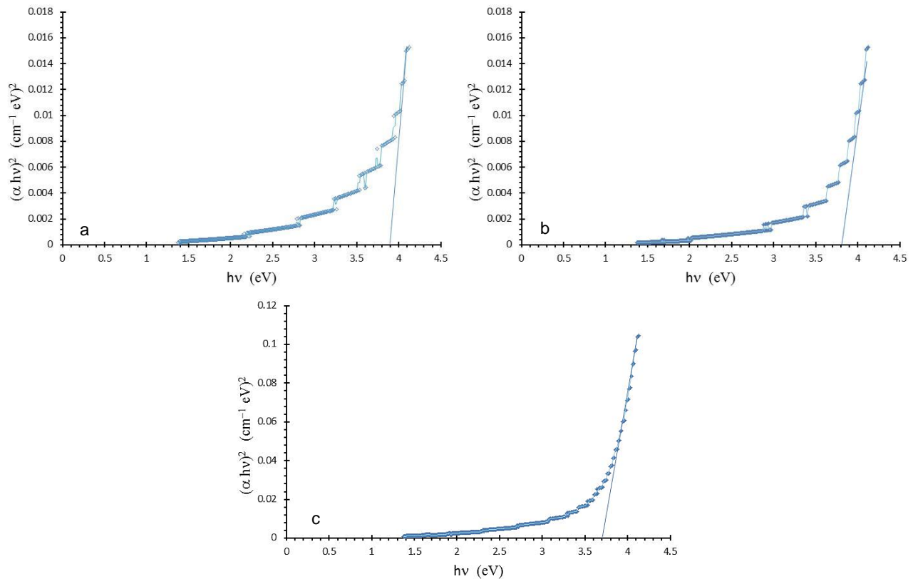
Figure 4: The optical band gap of TiO 2 NPs prepared at different laser energy (a) 80mJ (b) 120mJ, and (c) 160mJ.
