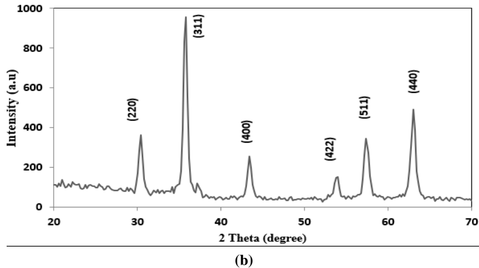
Figure 3: XRD of \text{Fe}_3\text{O}_4 (a) heating at 90^\circ\text{C} for 60 min.(b) heating at 400^\circ\text{C} for 120 min.
