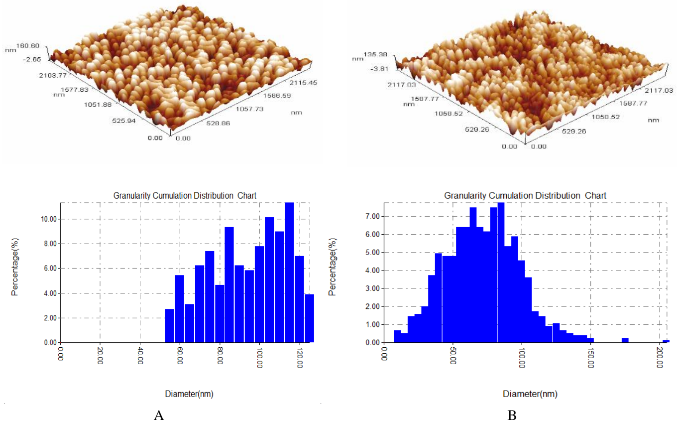
Figure 6: AFM images at 3D and Granularity accumulation distribution charts of \text{Fe}_3\text{O}_4 (a) as-prepared and (b) annealing, and \text{Fe}_2\text{O}_3 at 400 °C for 120 min respectively.
