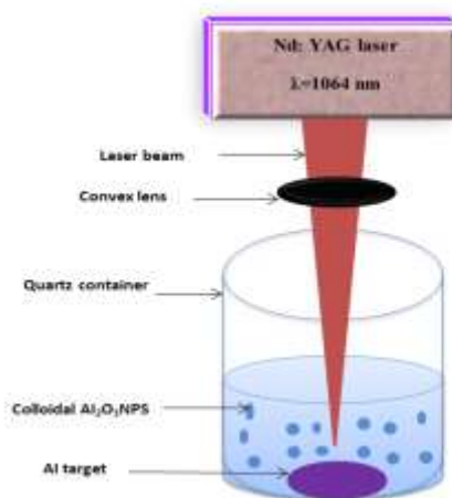
Figure 1: Setup for nanoparticle synthesis.
