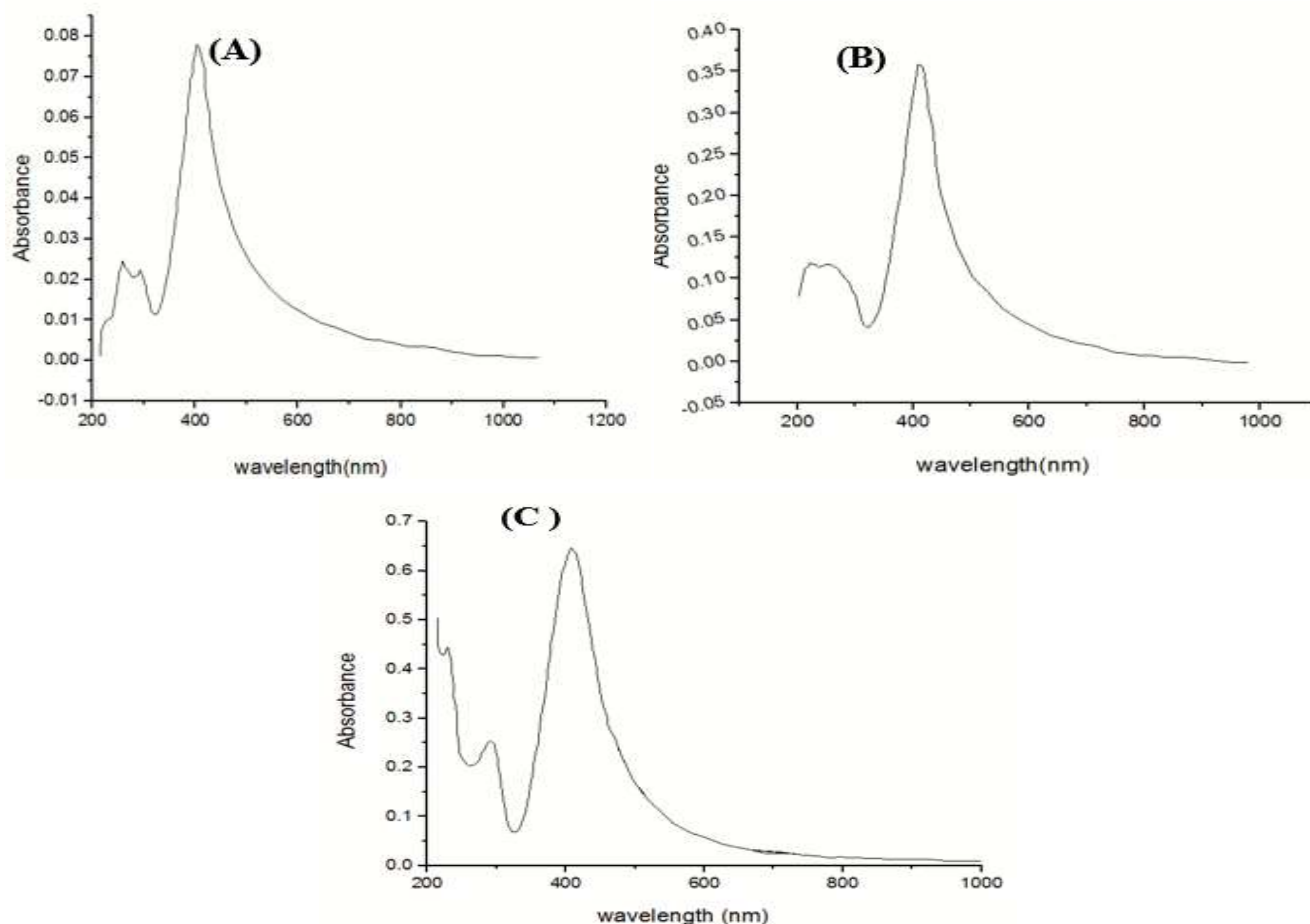
Figure 2: UV-Visible of Al 2 O 3 NPS at (A) 500 mJ, (B) 800 mJ, and (C) 1000 mJ energy.
