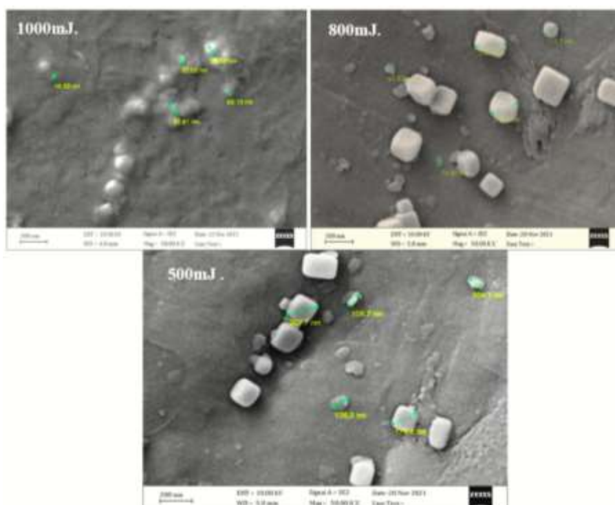
Figure 5: SEM image of Al 2 O 3 NPS at (A) 500mJ, (B) 800mJ, (C) 1000mJ energy.
