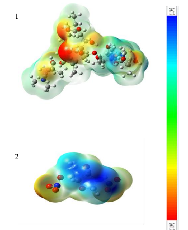
Figure 13: TED maps of the inhibitors.
