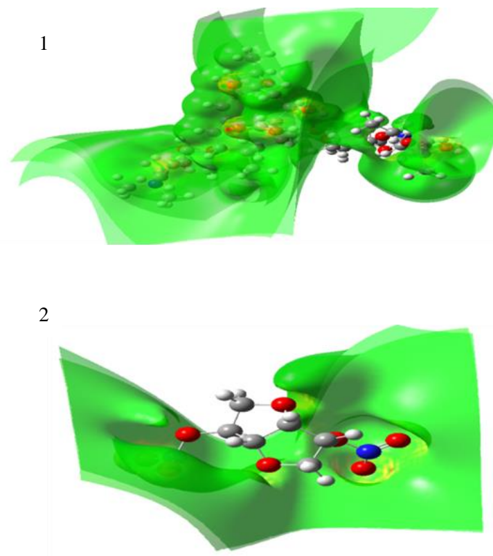
Figure 14: ESP map of the studied compounds.
