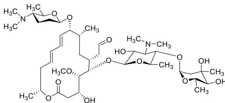
Figure 1: Chemical structure of Spiramycin structure.
