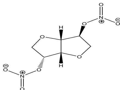
Figure 2: Chemical structure of Isosorbide dinitrate structure.
