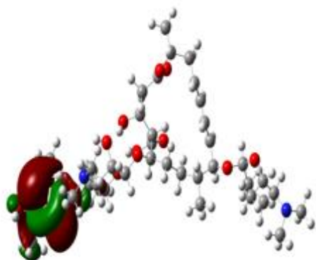
Figure 12: The energy levels (HOMO-LUMO) orbitals of the studied inhibitors (1 and 2).
