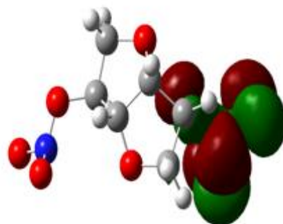
Figure 12: The energy levels (HOMO-LUMO) orbitals of the studied inhibitors (1 and 2).
