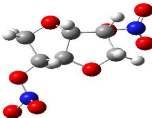
Figure 11: Equilibrium geometry of the inhibitors molecules calculated by DFT (B3LYP/6-311G (d,p)) method.
