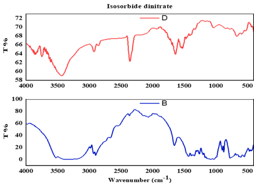
Figure 9: FTIR spectrum for Isosorbide dinitrate (blue line) and after adsorption on an aluminum surface, a film is formed (red line 200 ppm).
