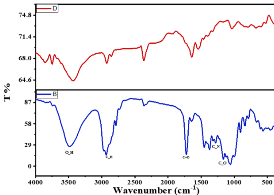
Figure 8: FTIR spectra of Spiramycin (blue line) and film formed after adsorption on aluminum surface (red line 200 ppm).
