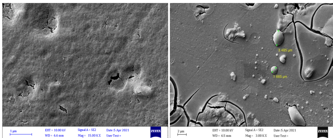
Figure 7: SEM images after inhibition with two inhibitors in HCl medium.
