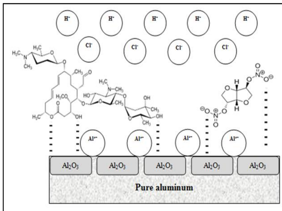
Figure 10: Mechanism of corrosion inhibition by drugs.
