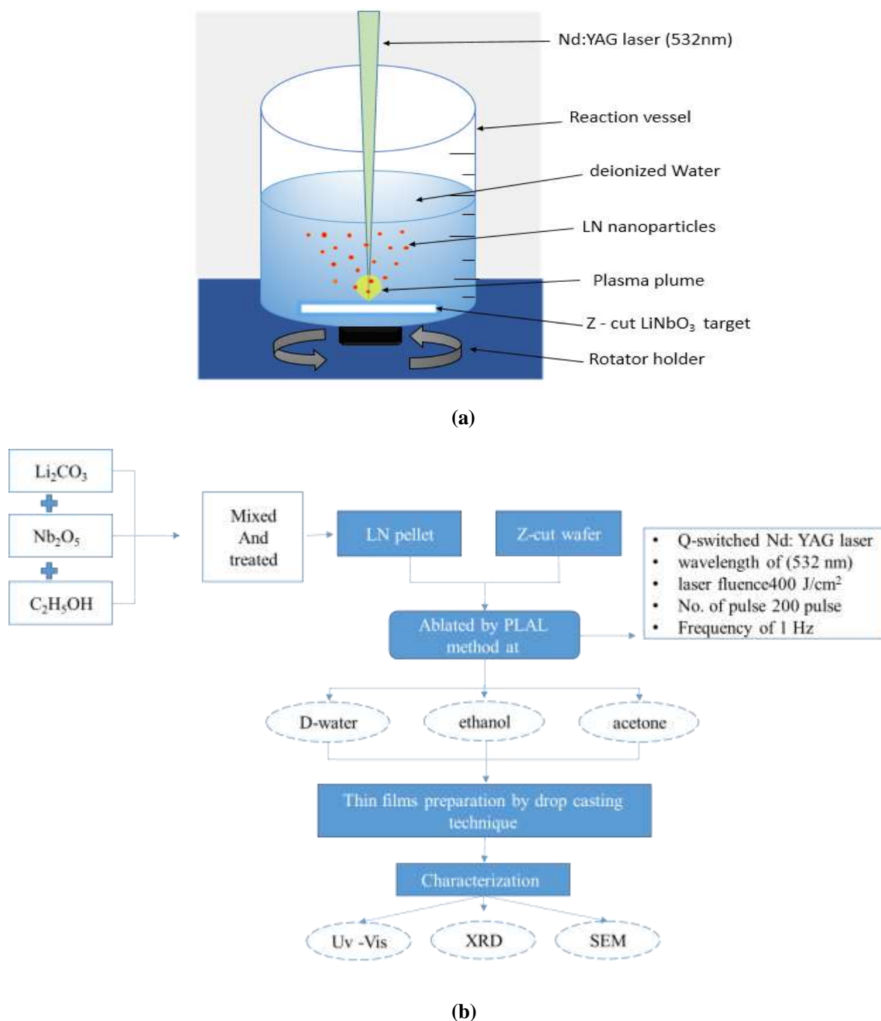
Figure 1: (a) Experimental setup on pulse laser ablation in liquid method, (b) bulk schematic diagram of preparation and characterization of the samples
