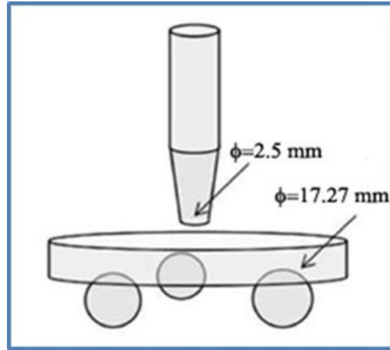
Figure 1: Piston-on-three ball biaxial flexural strength test [11].
