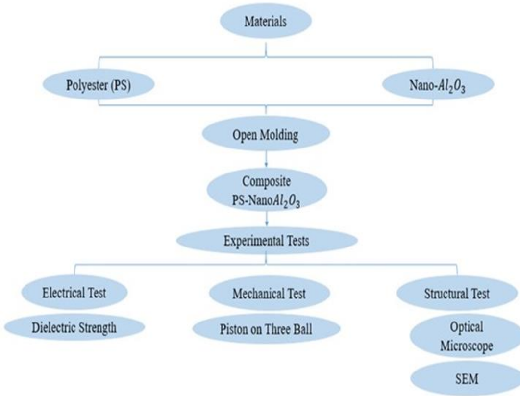
Figure 2: Methodology of Procedure.
