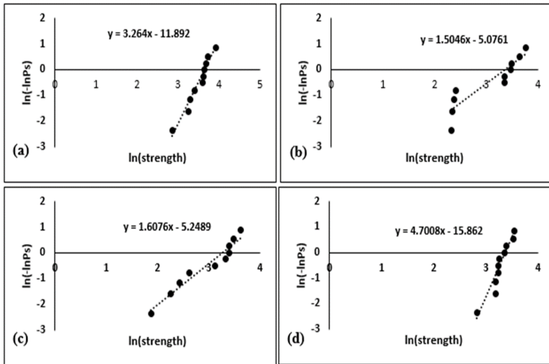
Figure 3: Weibull Distribution by piston-on-three-ball test (a) 1 wt% Al_2O_3 , (b) 2 wt% Al_2O_3 , (c) 3 wt% Al_2O_3 , (d) 4 wt% Al_2O_3 .
