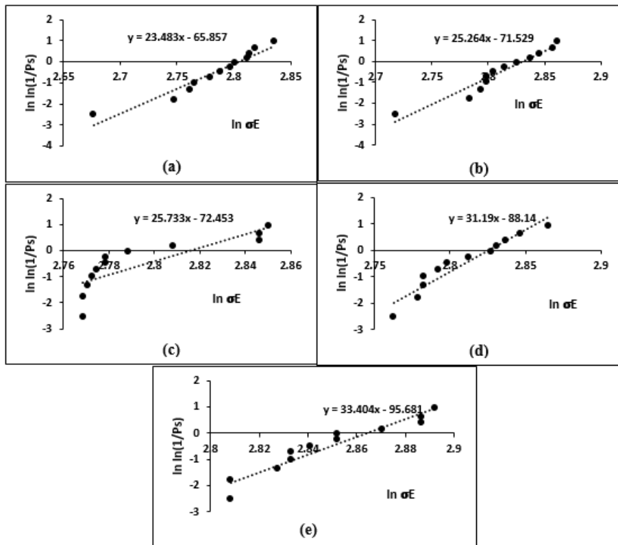
Figure 7: Weibull distribution of dielectric strength at various RRV: (a) 0.5, (b) 1, (c) 2, (d) 3 and (e) 5 kV/s, for 3 wt% Al 2 O 3 .
