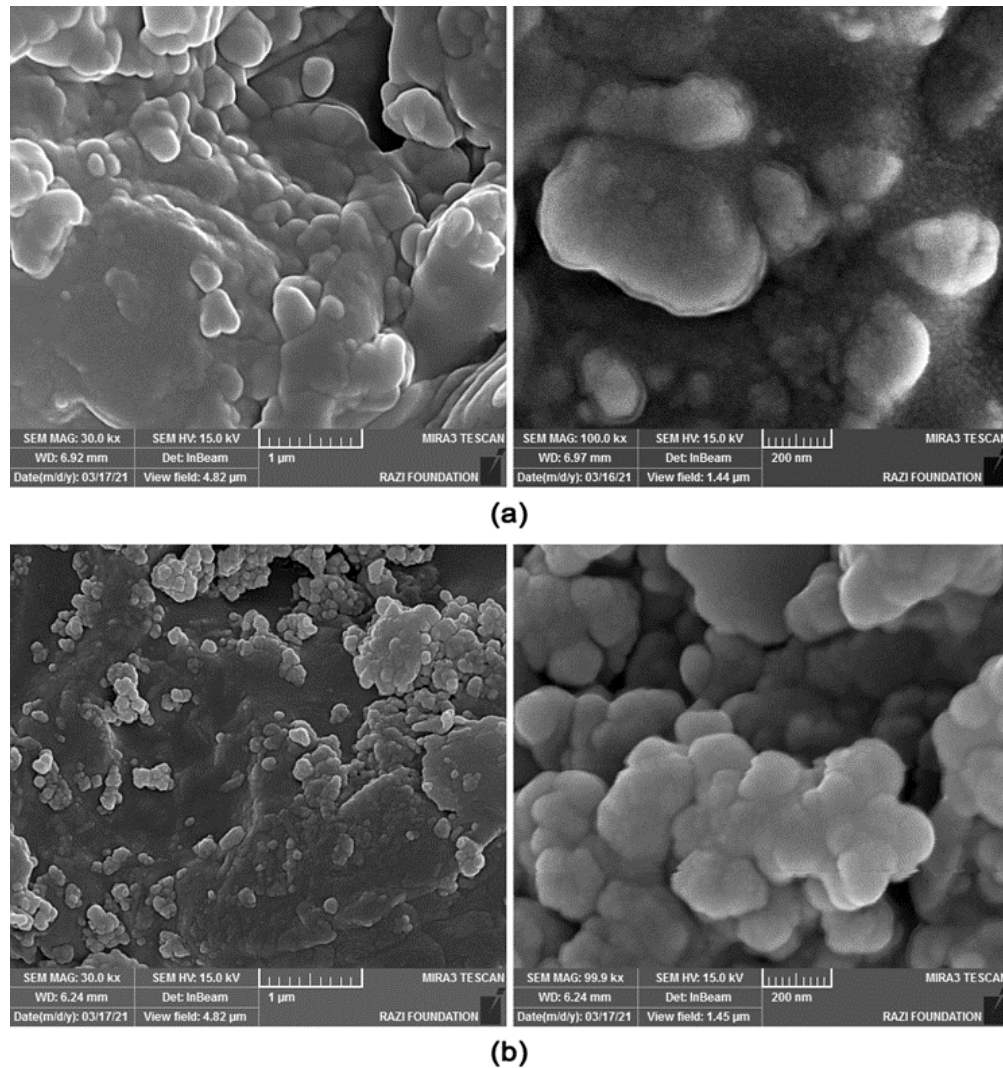
Figure 11: SEM image of PS with (a) 1% \text{Al}_2\text{O}_3 and (b) 4% \text{Al}_2\text{O}_3 composites.
