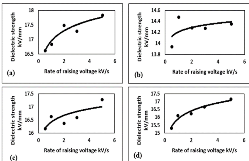
Figure 4: Variation of dielectric strength with RRV for (a) 1 wt% \text{Al}_2\text{O}_3 (b) 2 wt% \text{Al}_2\text{O}_3 (c) 3 wt% \text{Al}_2\text{O}_3 and (d) 4 wt% \text{Al}_2\text{O}_3 .
