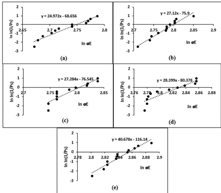
Figure 8: Weibull distribution of dielectric strength at various RRV: (a) 0.5, (b) 1, (c) 2, (d) 3 and (e) 5 kV/s, for 4 wt% Al 2 O 3 .
