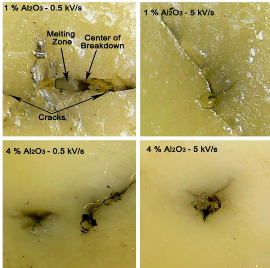
Figure 9: Trace of electrical breakdown damage for 1% Al 2 O 3 and 4% Al 2 O 3 with 0.5, 5 kV/s.
