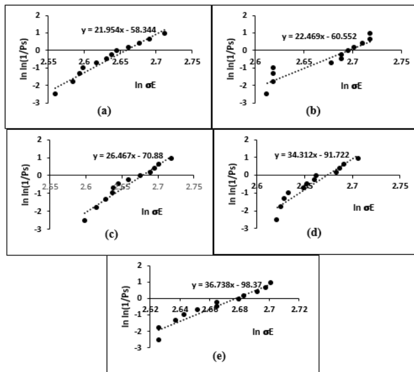
Figure 6: Weibull distribution of dielectric strength at various RRV: (a) 0.5, (b) 1, (c) 2, (d) 3 and (e) 5 kV/s, for 2 wt% Al 2 O 3 .
