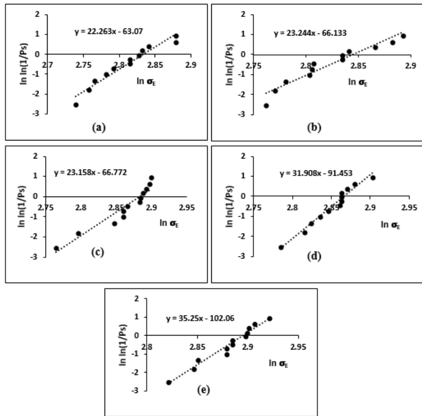
Figure 5: Weibull distribution of dielectric strength at various RRV: (a) 0.5, (b) 1, (c) 2, (d) 3 and (e) 5 kV/s, for 1 wt% Al 2 O 3 .
