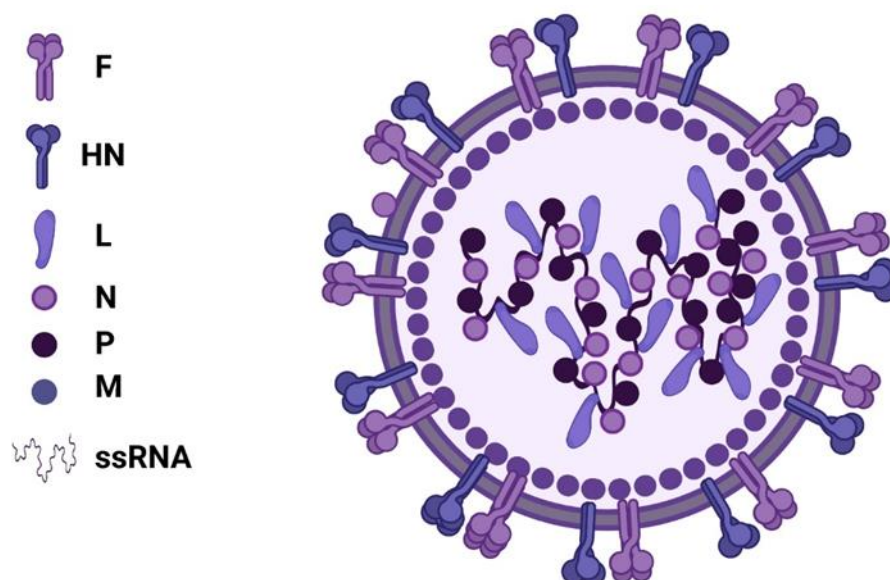
Figure 1: Schematic diagram of Newcastle disease virus structure. This figure was created using BioRender tools by the authors
