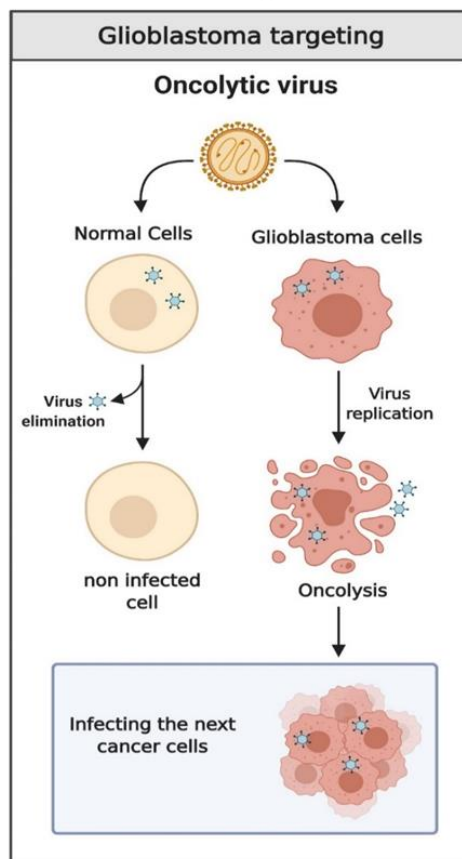
Figure 8: The proposed mechanism for NDV-AMHA1 strain against Iraqi patient-derived glioblastoma multiforme.
