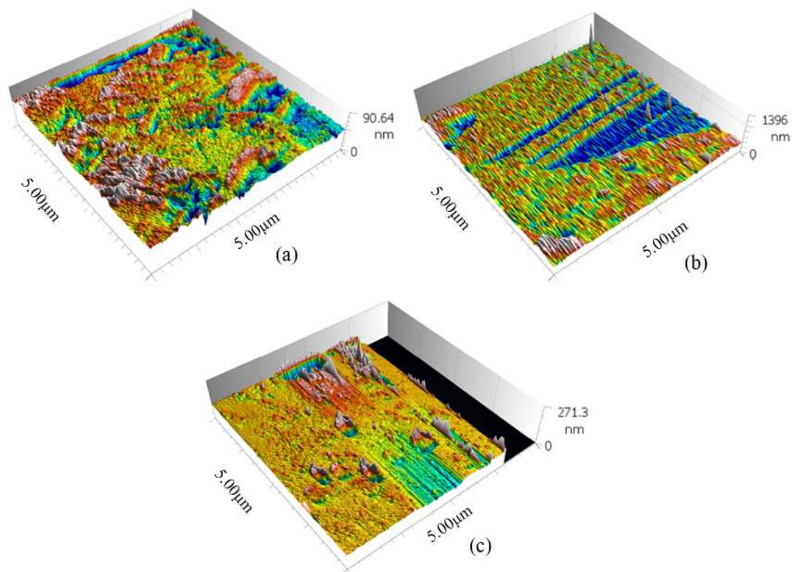
Figure 8: AFM at a magnification ( 5.00 \mu\text{m} \times 5.00 \mu\text{m} ) of precursor after chemical activation (a) PPK1, (b) PPK2, and (c) PPK3.
